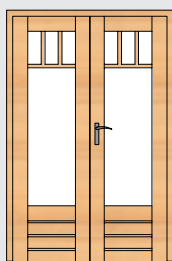
PE41 1210 x 1800 PE41H 1210 x 1935
