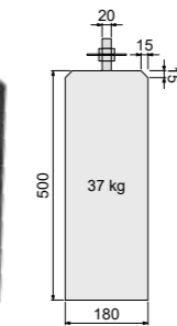
Betonpoer antraciet
